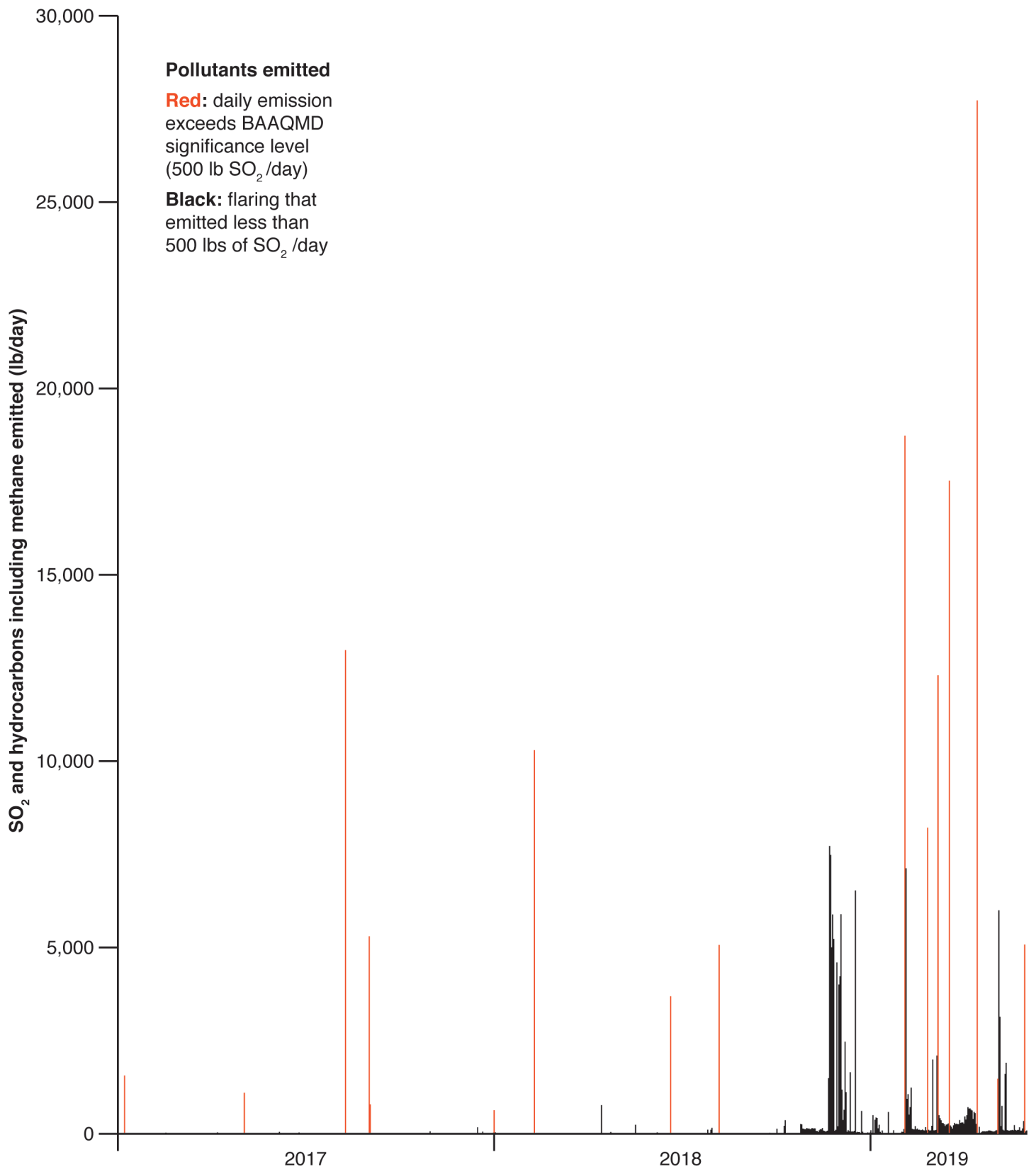
Daily emissions from flares, Chevron Richmond Refinery, January 2017—May 2019. SO 2 : Sulfur dioxide. lb/day: pounds per day. Data from www.BAAQMD.gov ; chart by CBE.
