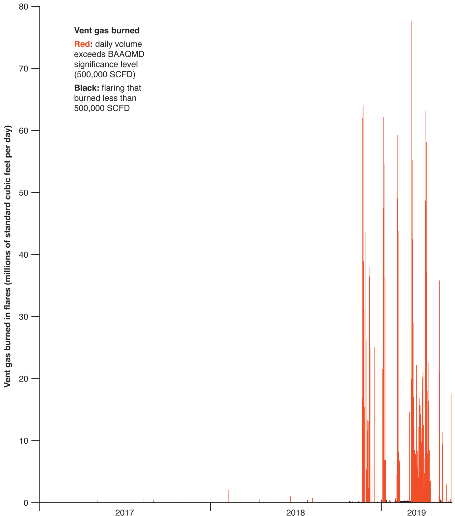
Daily vent gas volume flared, Chevron Richmond Refinery, January 2017—May 2019. SCFD: Standard cubic feet per day. Data from www.BAAQMD.gov ; chart by CBE. See emissions, next page.
