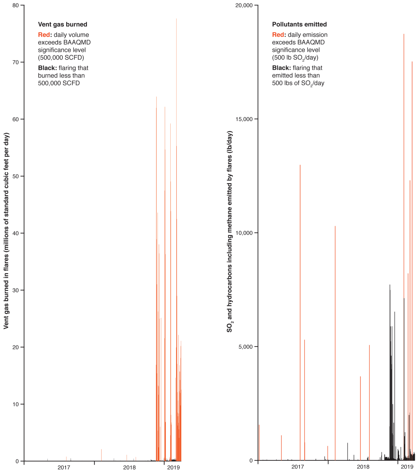
Daily vent gas volume flared and emissions from flares, Chevron Richmond Refinery, January 2017—March 2019. SCF: Standard cubic feet. SO 2 : Sulfur dioxide. lb/day: pounds per day. Data from www.BAAQMD.gov ; charts by CBE.
